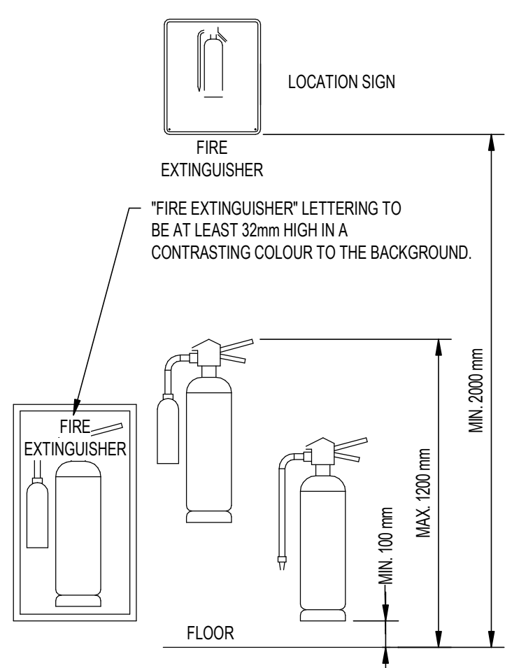
FIRE EXTINGUISHER MOUNTING HEIGHT AND SIGNAGE DETAIL 1:20
