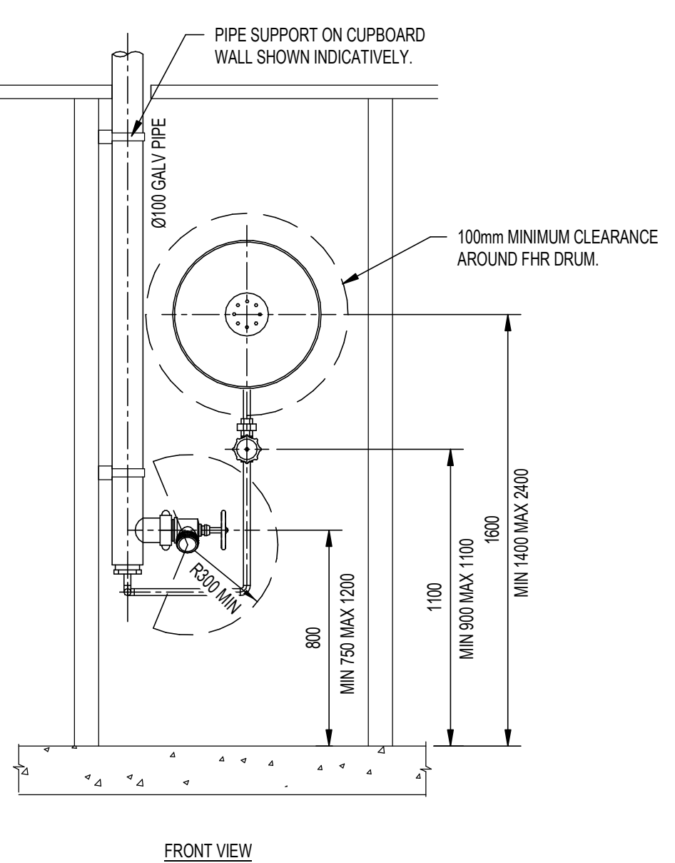
HYDRANT & HOSE REEL CUPBOARD DETAIL 1:20
