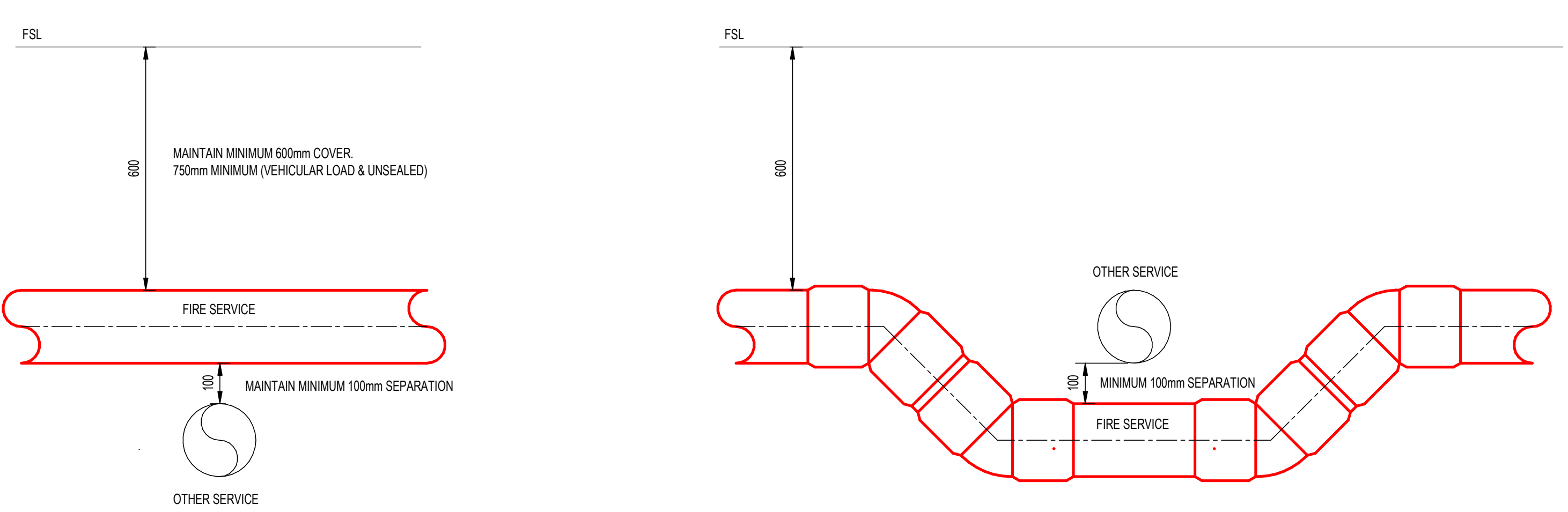
MINIMUM DEPTH OF COVER FOR BURIED PIPES 1:10
