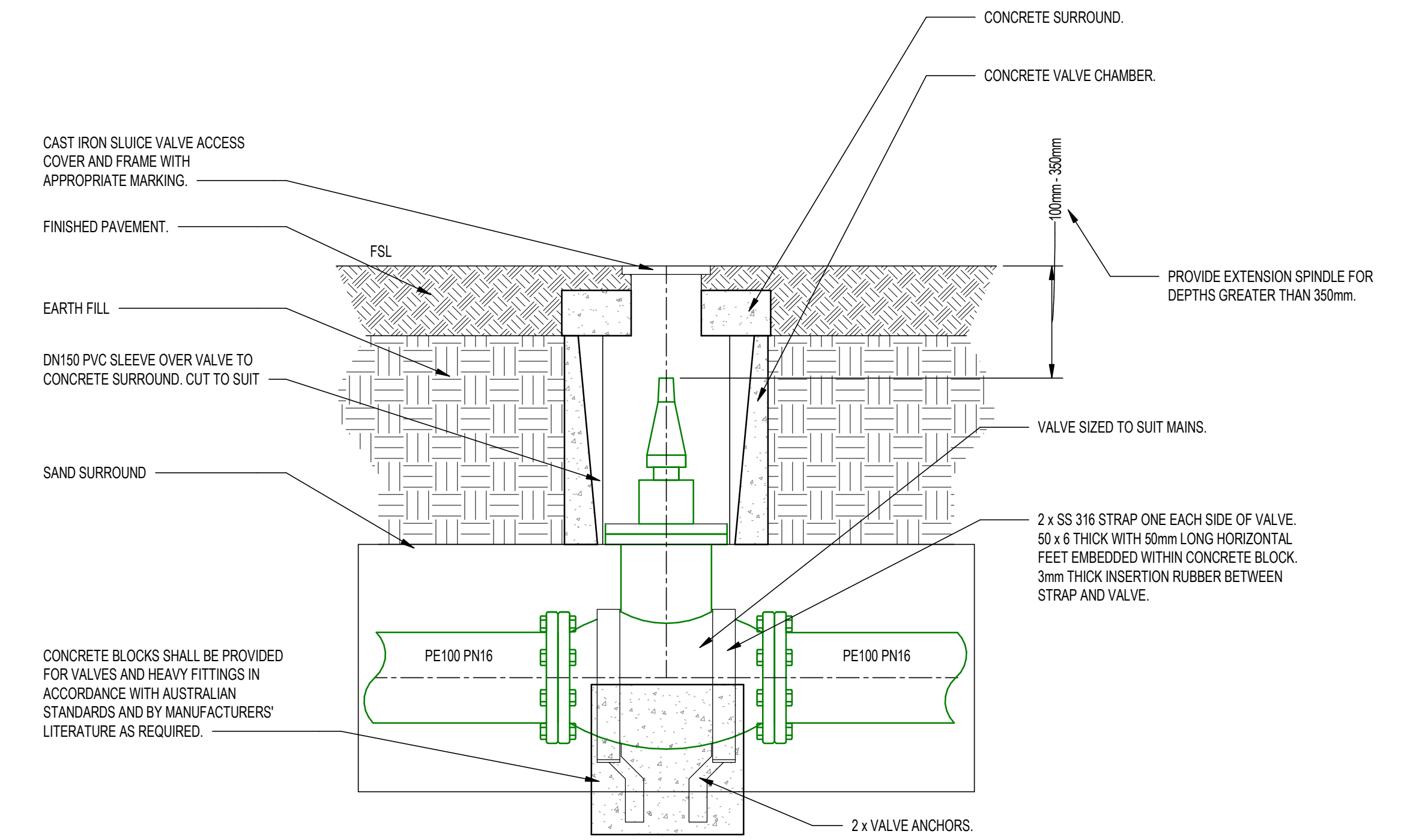
TRAFFICABLE BELOW GROUND SLUICE VALVE DETAIL 1:10
