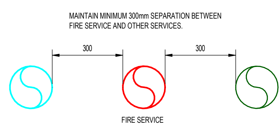
BURIED PIPES MINIMUM HORIZONTAL SEPARATION REQUIREMENTS PARALLEL TRENCH 1:10
