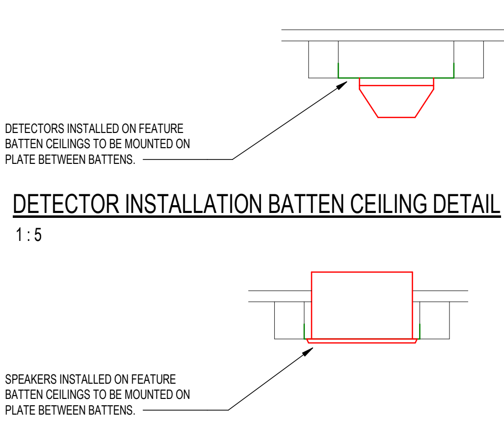
DETECTOR INSTALLATION BATTEN CEILING DETAIL 1:5
