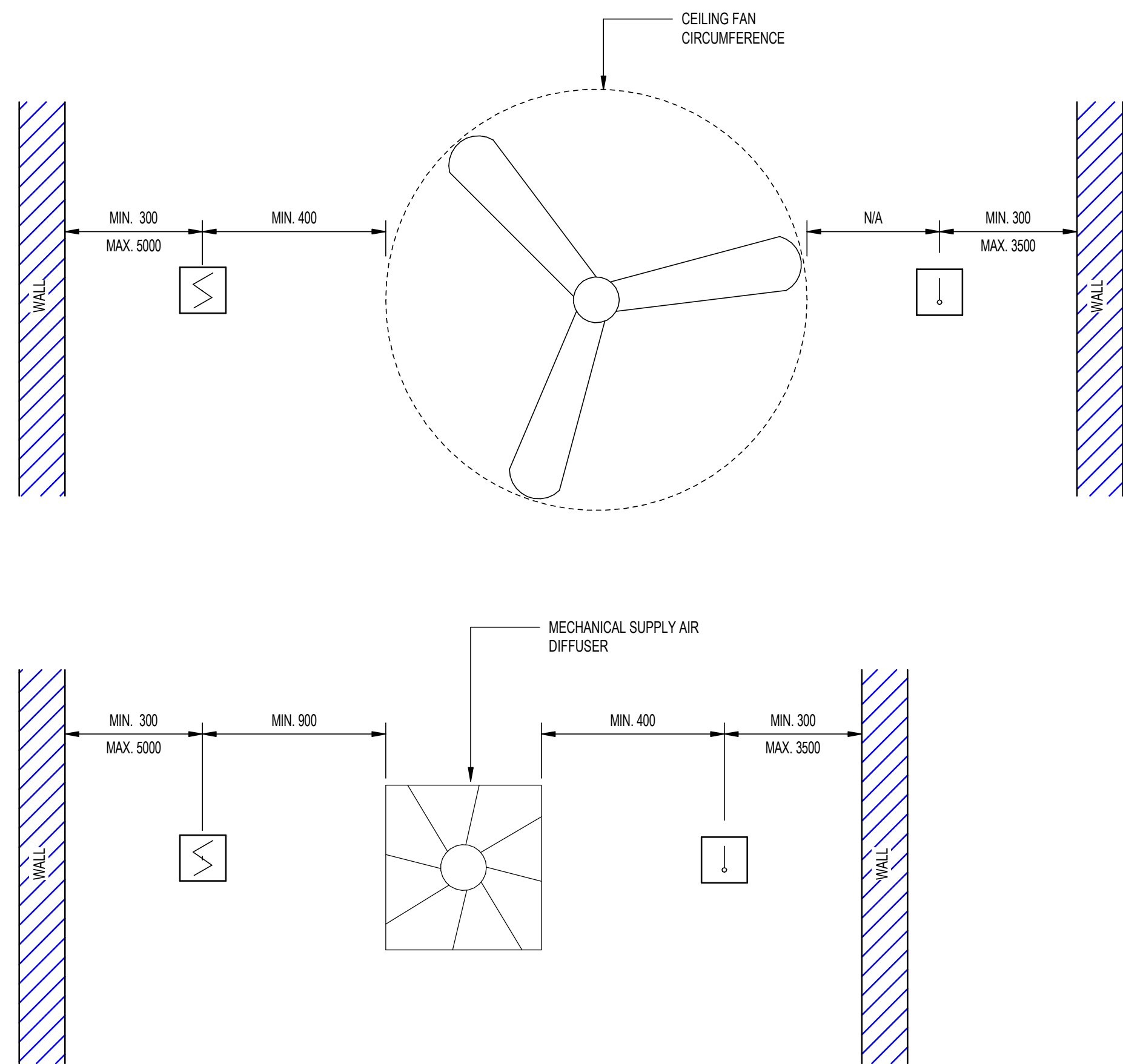
STANDARD FIRE DETECTION SPACING REQUIREMENTS 1:10
