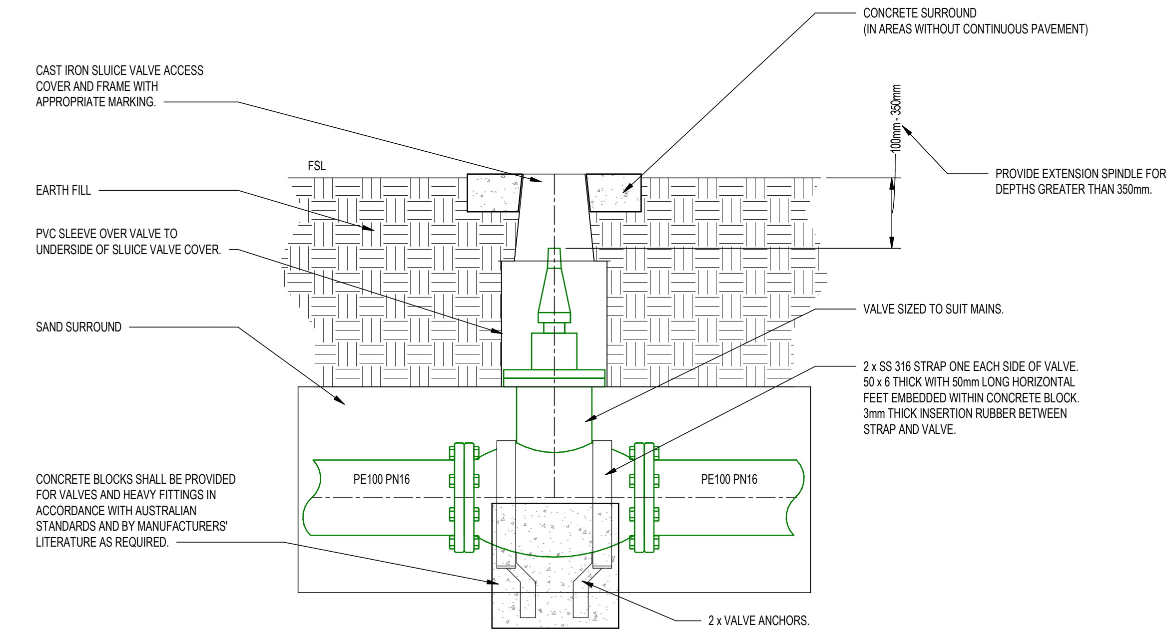
NON-TRAFFICABLE BELOW GROUND SLUICE VALVE DETAIL 1:10
