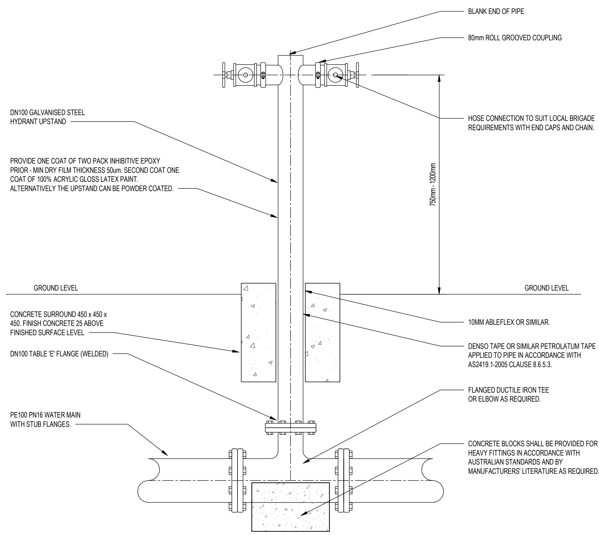
DOUBLE PILLAR ATTACK HYDRANT DETAIL 1:10
