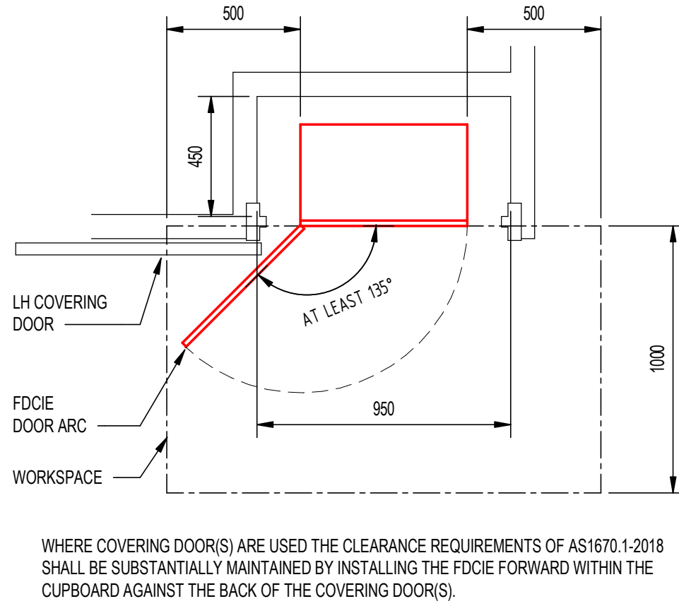
FDCE FIRE PANEL CUPBOARD DETAIL 1:20
