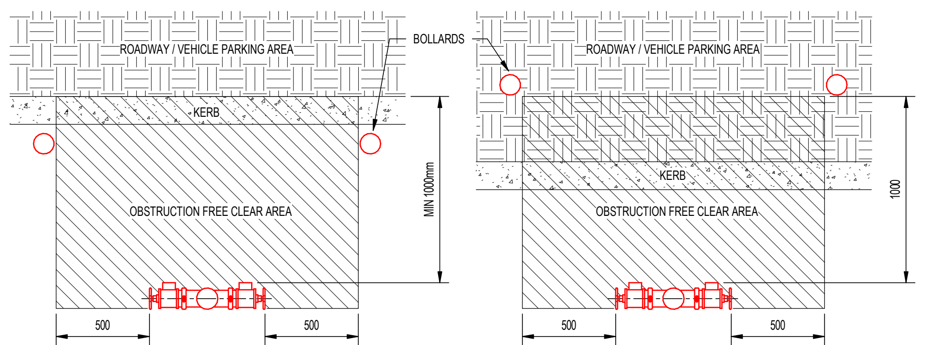
DOUBLE PILLAR EXTERNAL HYDRANT BOLLARDS DETAIL 1:20
