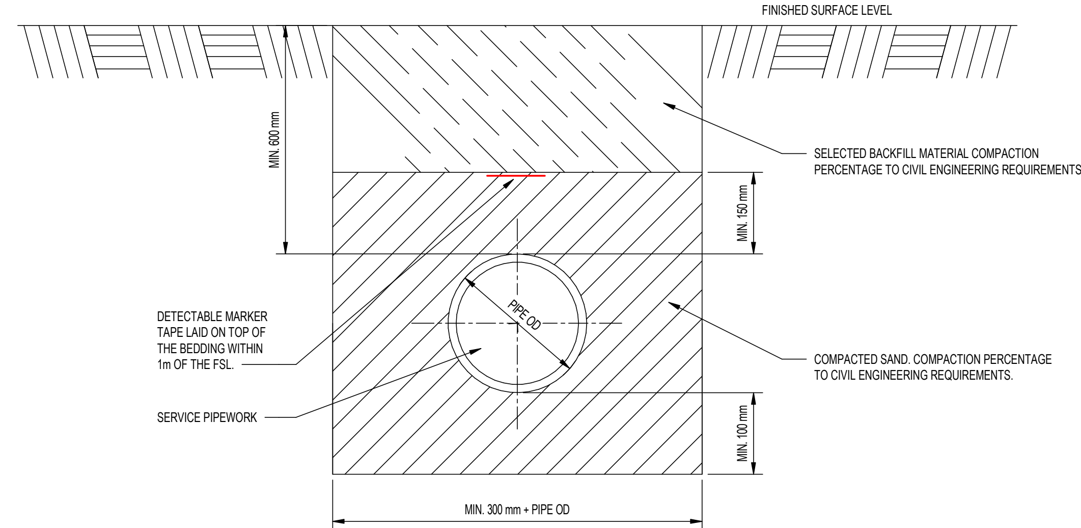
UNDERGROUND FIRE SERVICES TRENCH DETAIL 1:5
